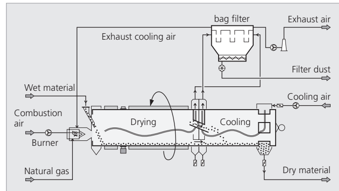
Separate extraction of the exhaust air streams and heat recovery
